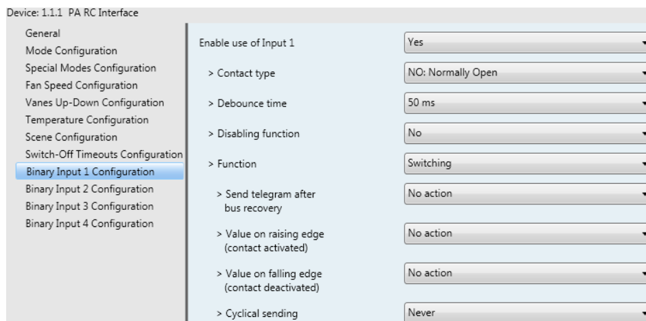
Figure 4.37 Binary Input Configuration dialog
